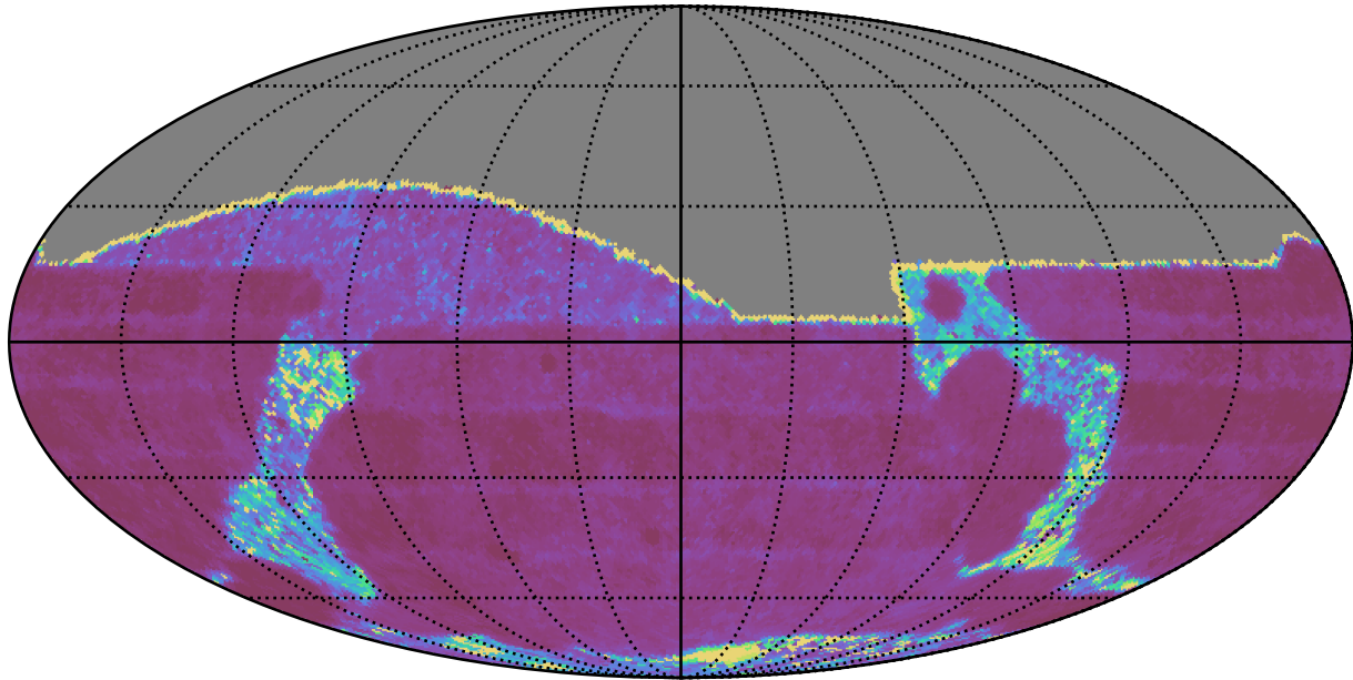
weather_cloudso4v3.4_10yrs All sky g band: Median Inter-Night Gap
