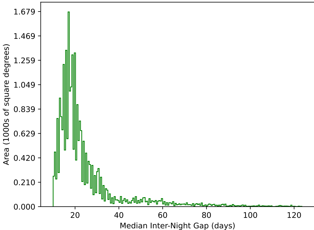
weather_cloudso4v3.4_10yrs All sky g band: Median Inter-Night Gap
