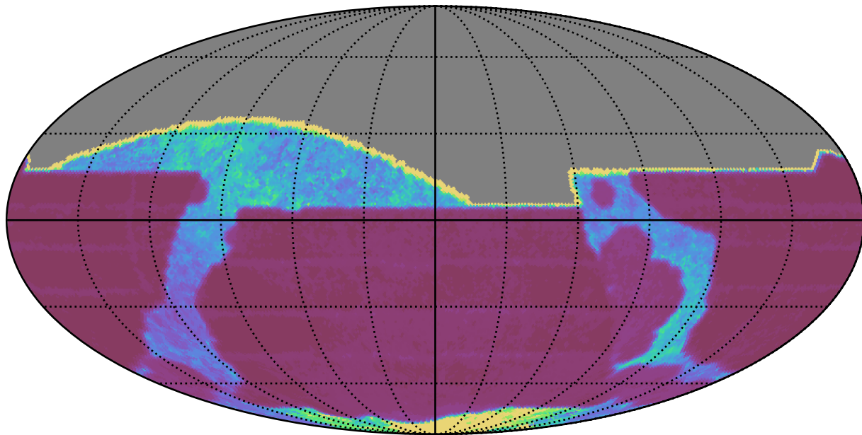
weather_cloudso4v3.4_10yrs All sky all bands: Median Inter-Night Gap
