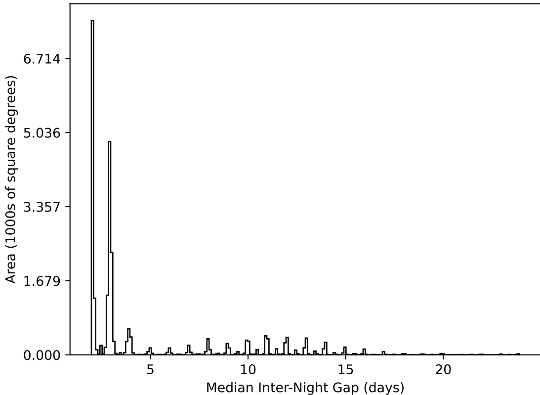
weather_cloudso4v3.4_10yrs All sky all bands: Median Inter-Night Gap
