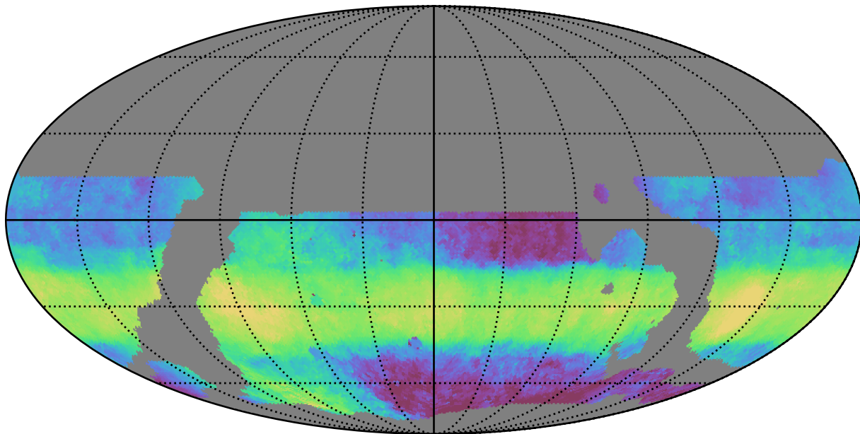
weather_cloudso4v3.4_10yrs WFD z band: Median HA
