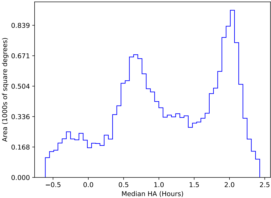
weather_cloudso4v3.4_10yrs WFD z band: Median HA
