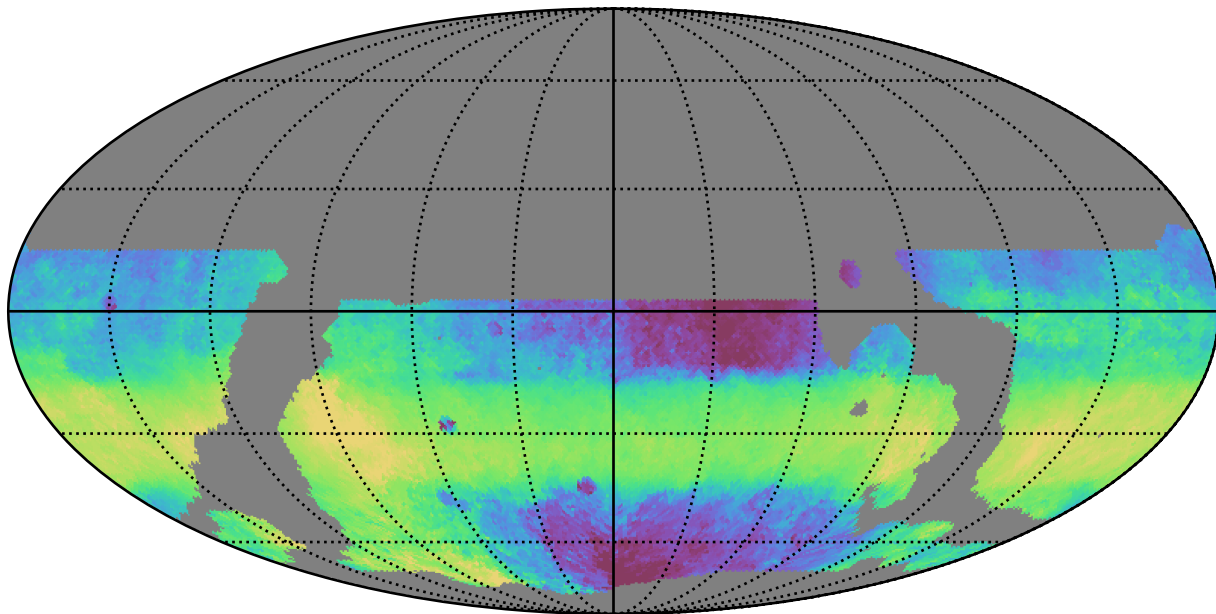
weather_cloudso4v3.4_10yrs WFD y band: Median HA
