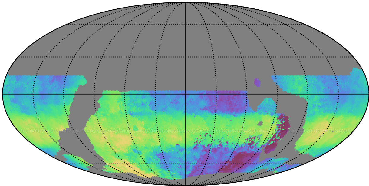
weather_cloudso4v3.4_10yrs WFD u band: Median HA
