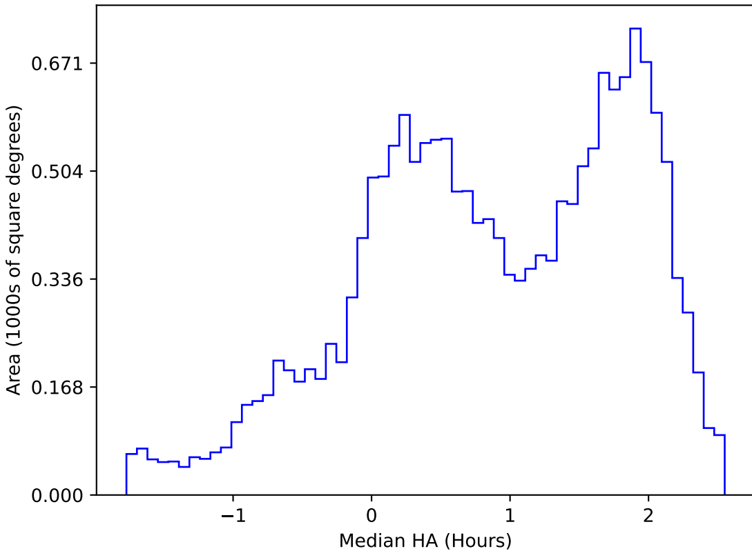
weather_cloudso4v3.4_10yrs WFD u band: Median HA
