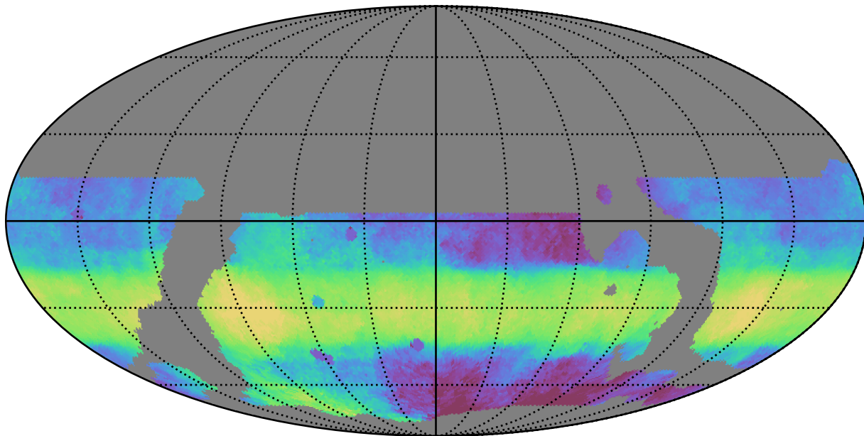
weather_cloudso4v3.4_10yrs WFD i band: Median HA
