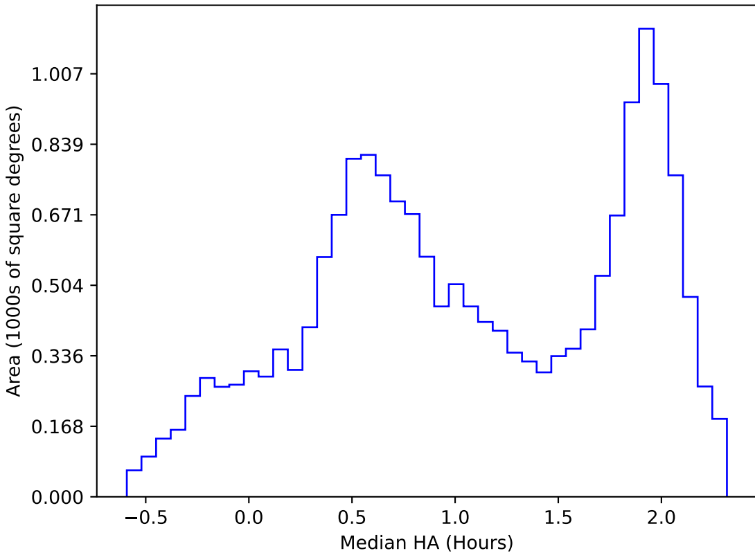
weather_cloudso4v3.4_10yrs WFD i band: Median HA
