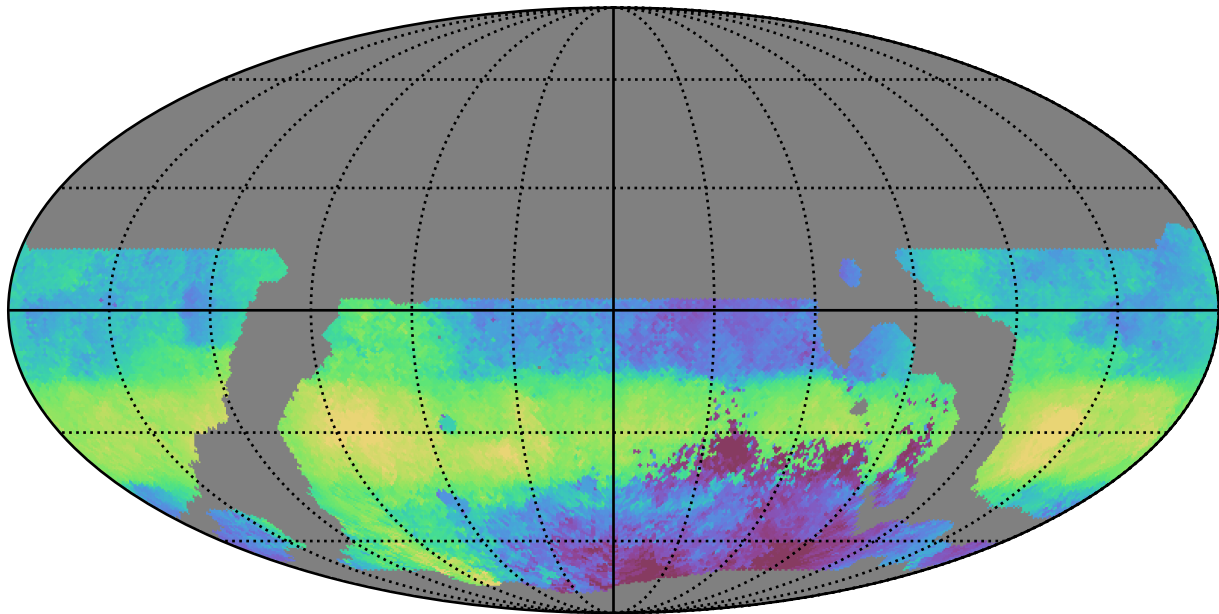
weather_cloudso4v3.4_10yrs WFD g band: Median HA
