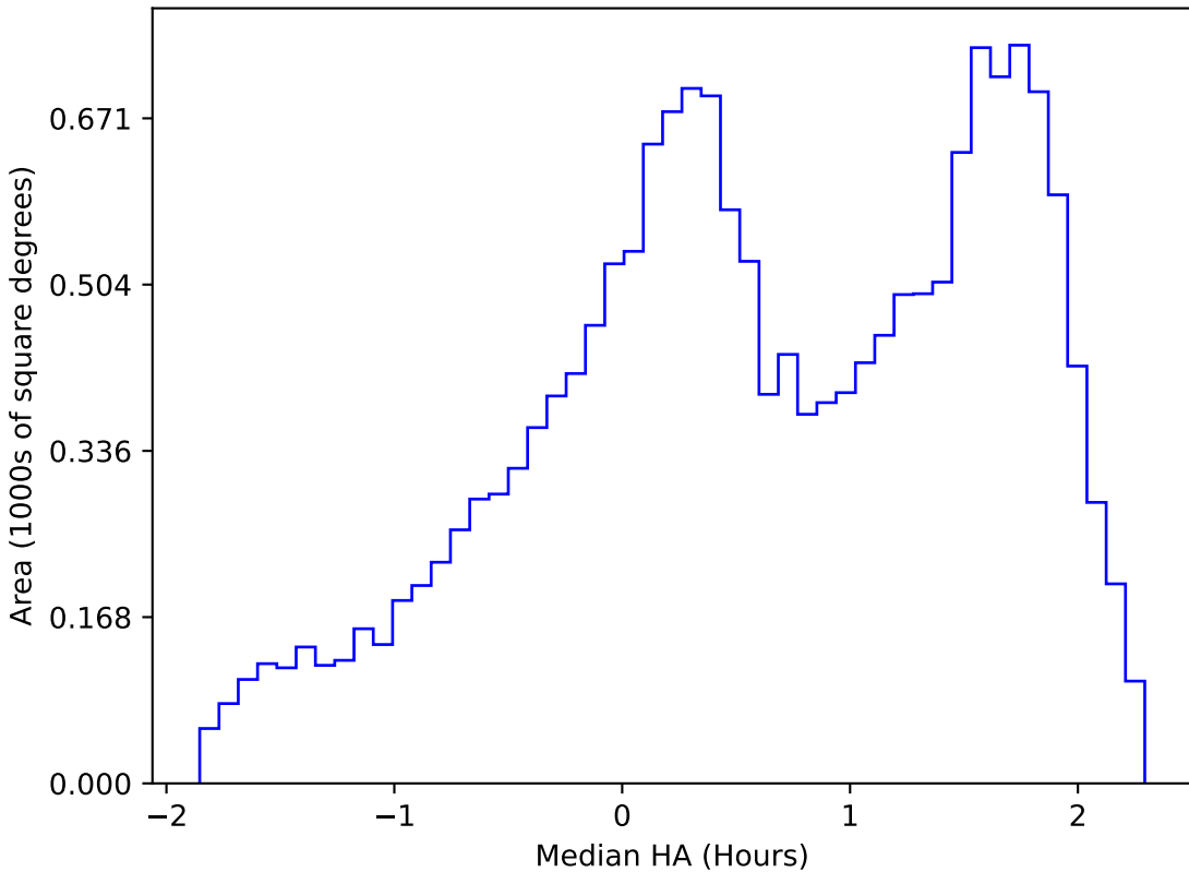
weather_cloudso4v3.4_10yrs WFD g band: Median HA
