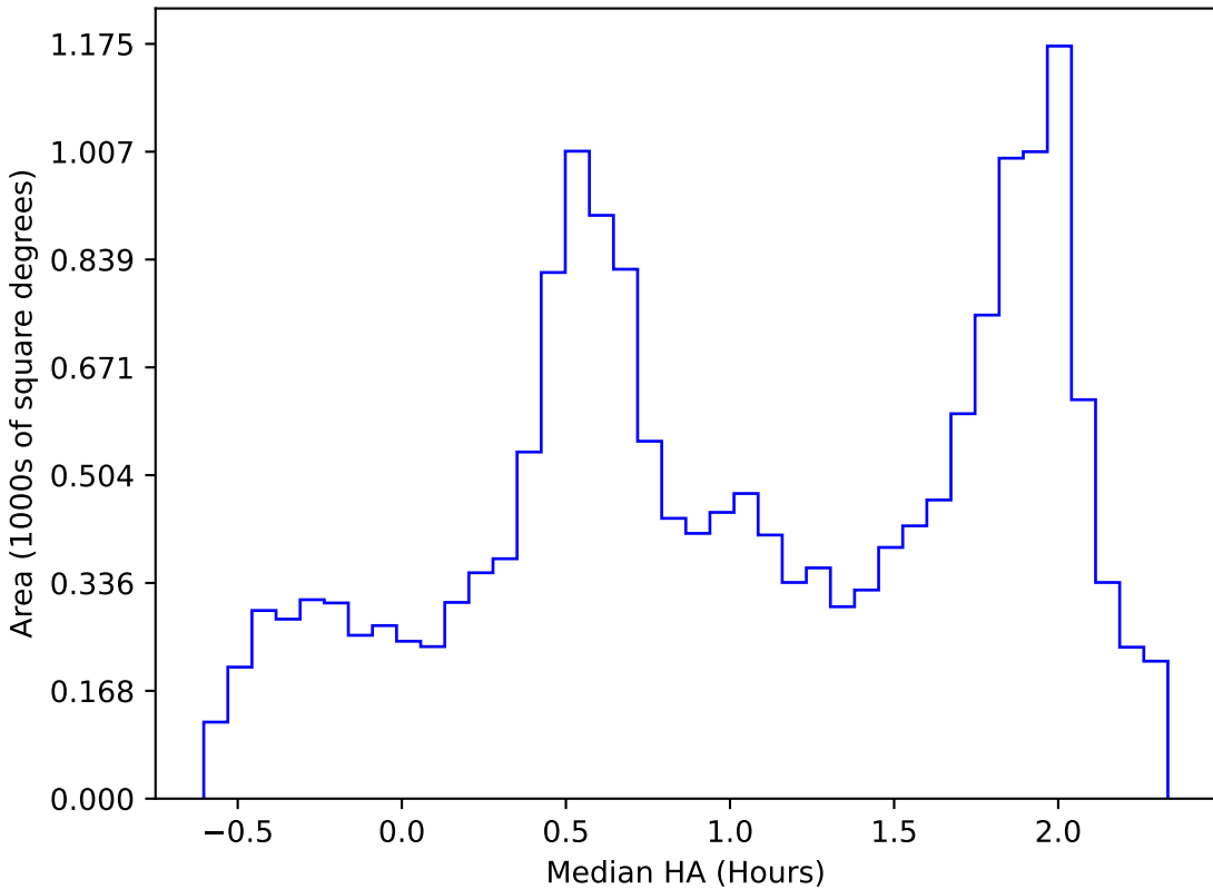
weather_cloudso4v3.4_10yrs WFD all bands: Median HA
