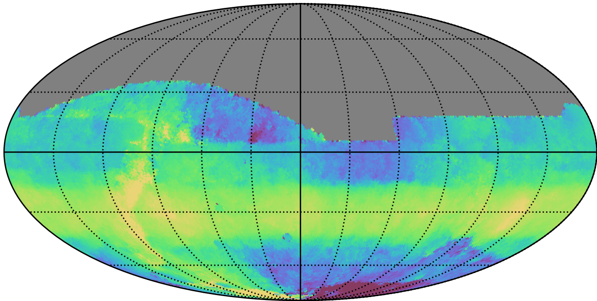
weather_cloudso4v3.4_10yrs All sky z band: Median HA
