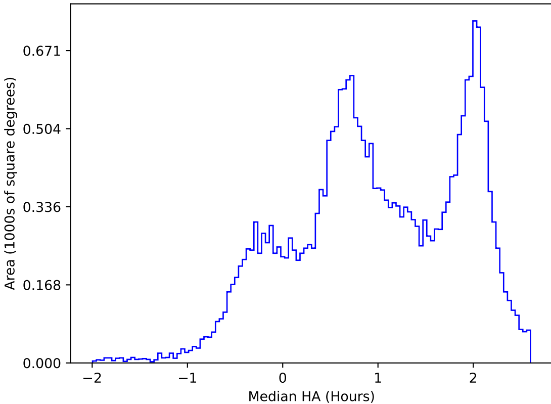
weather_cloudso4v3.4_10yrs All sky z band: Median HA
