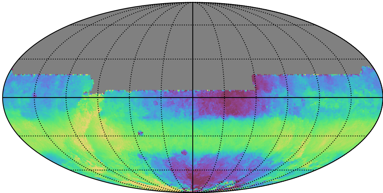
weather_cloudso4v3.4_10yrs All sky y band: Median HA
