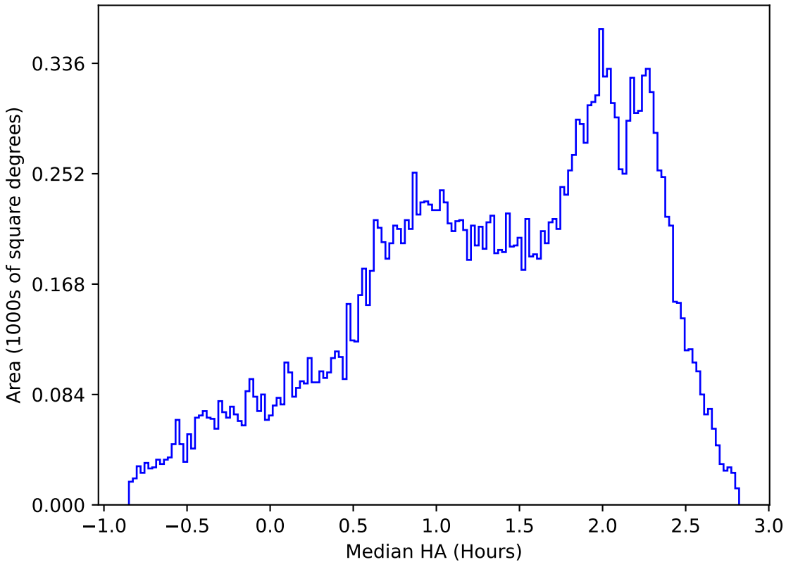
weather_cloudso4v3.4_10yrs All sky y band: Median HA
