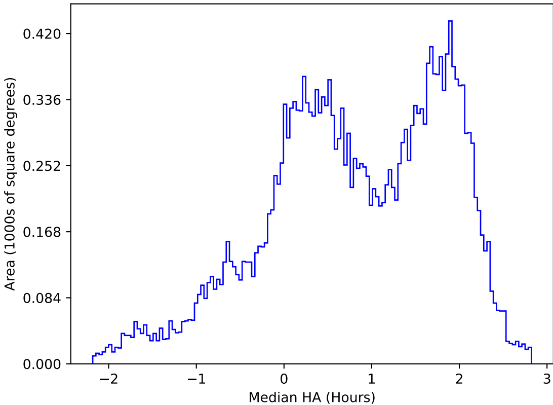
weather_cloudso4v3.4_10yrs All sky u band: Median HA
