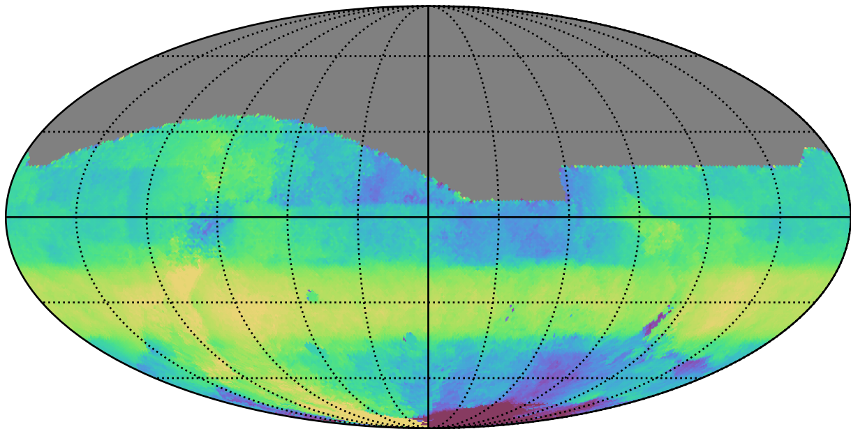
weather_cloudso4v3.4_10yrs All sky r band: Median HA
