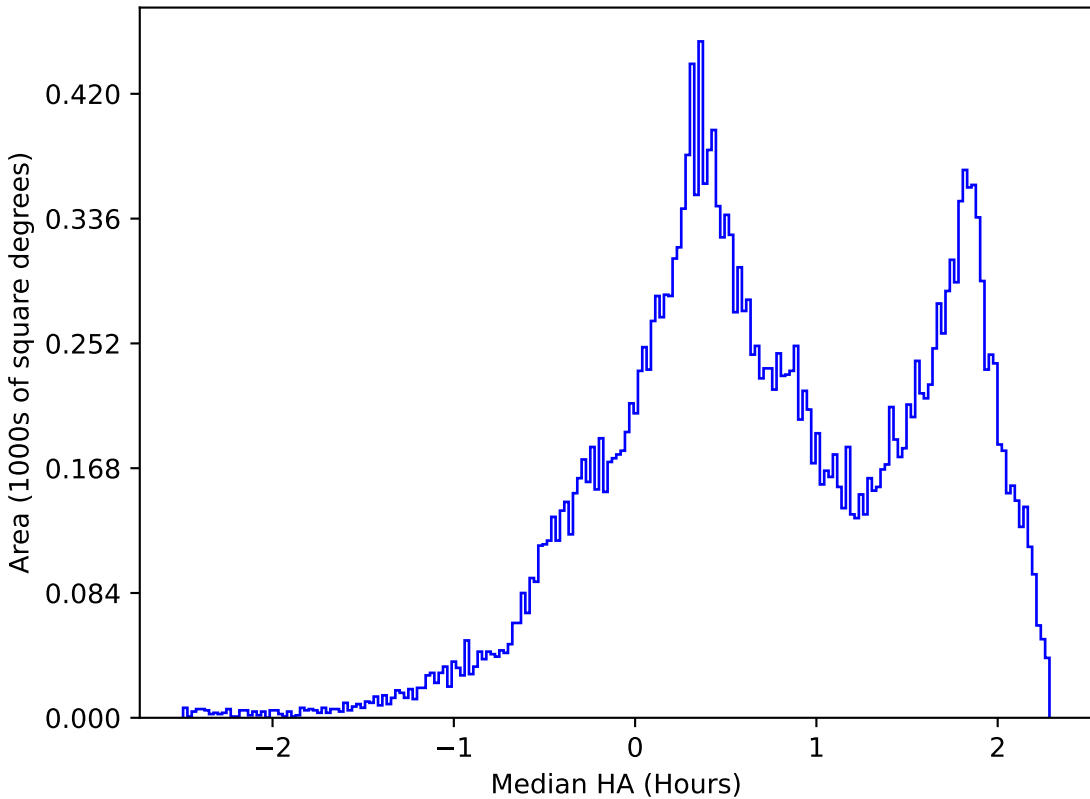
weather_cloudso4v3.4_10yrs All sky r band: Median HA
