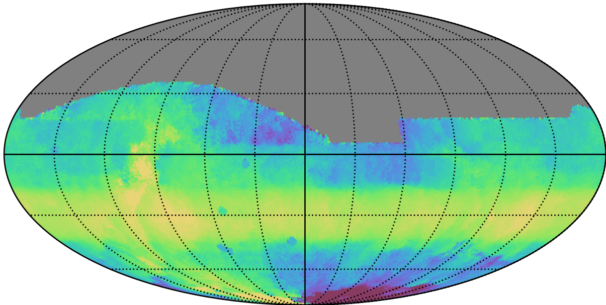
weather_cloudso4v3.4_10yrs All sky i band: Median HA
