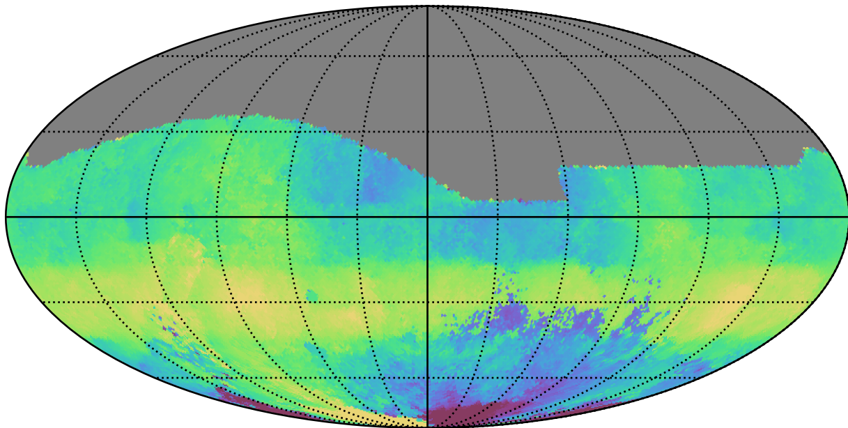
weather_cloudso4v3.4_10yrs All sky g band: Median HA
