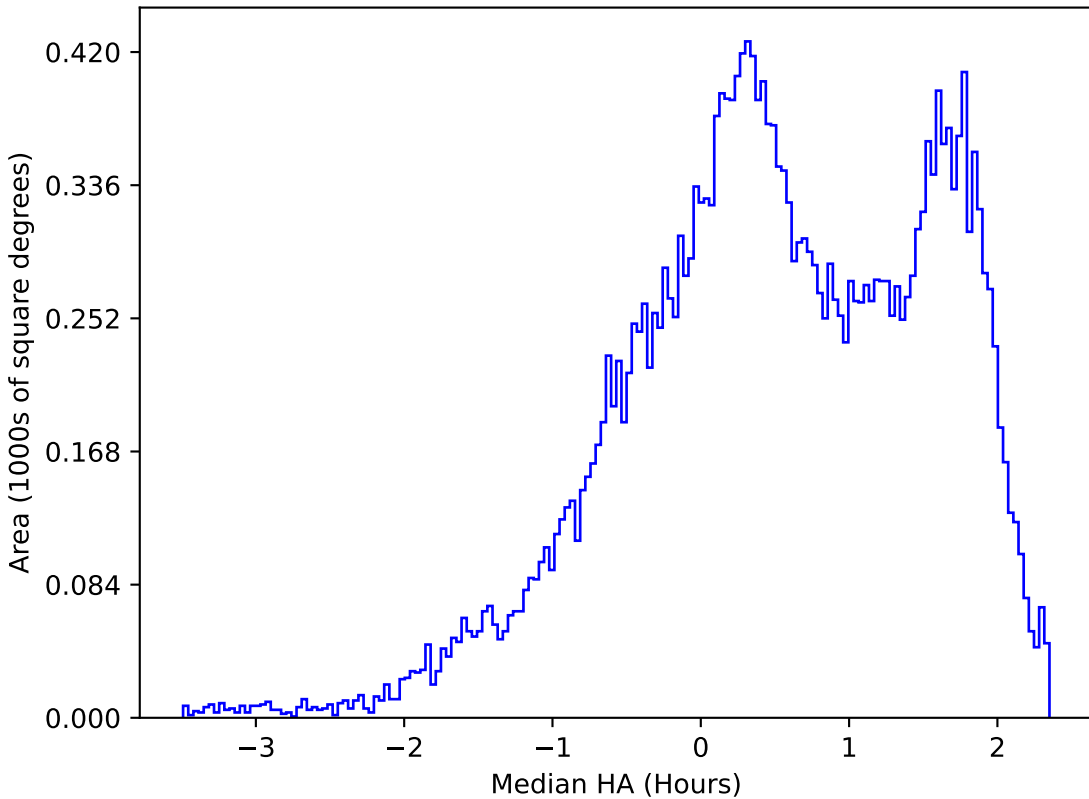
weather_cloudso4v3.4_10yrs All sky g band: Median HA
