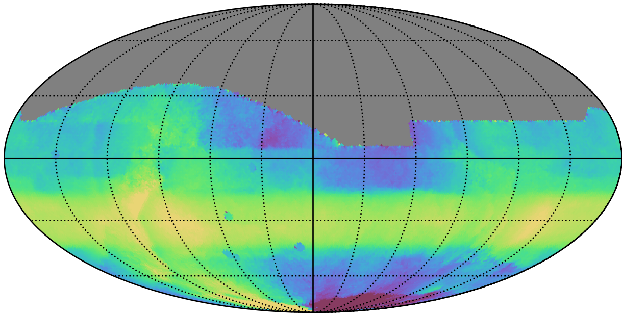
weather_cloudso4v3.4_10yrs All sky all bands: Median HA
