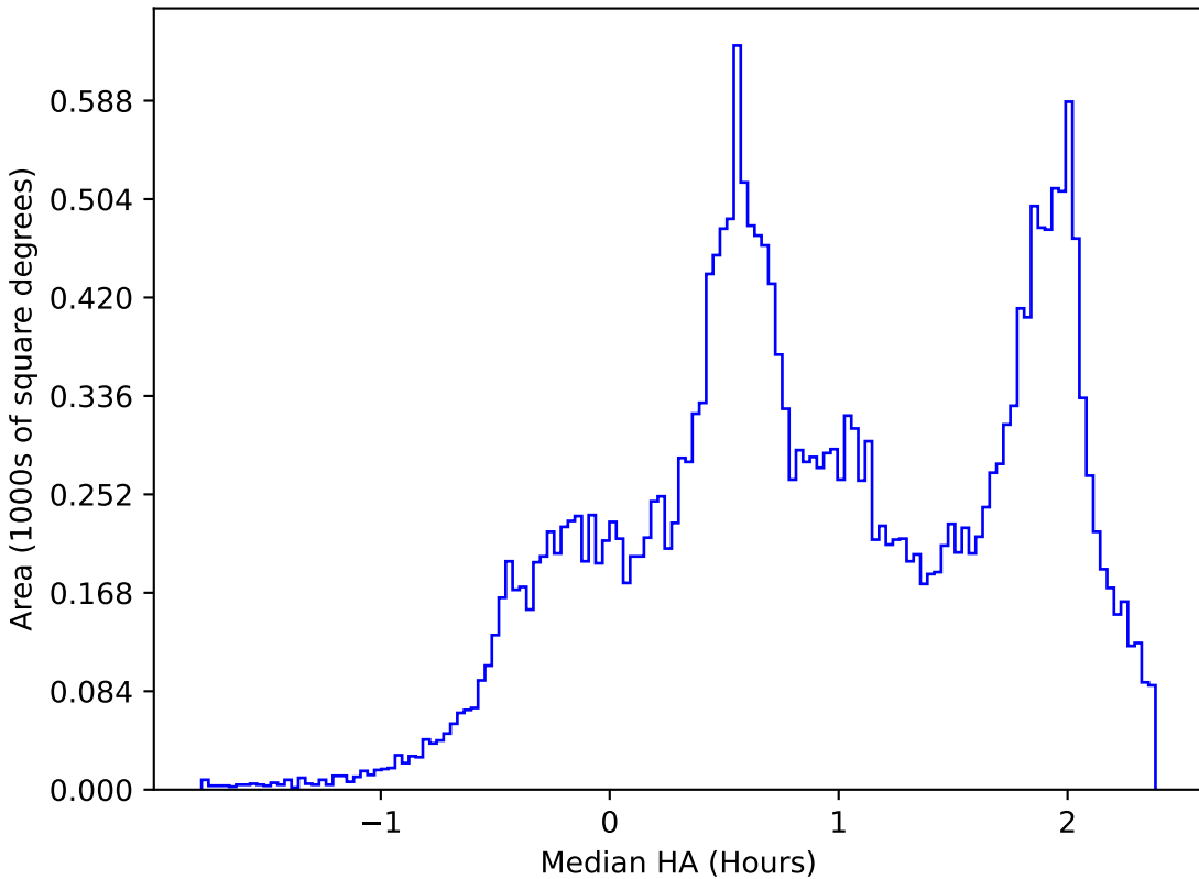
weather_cloudso4v3.4_10yrs All sky all bands: Median HA
