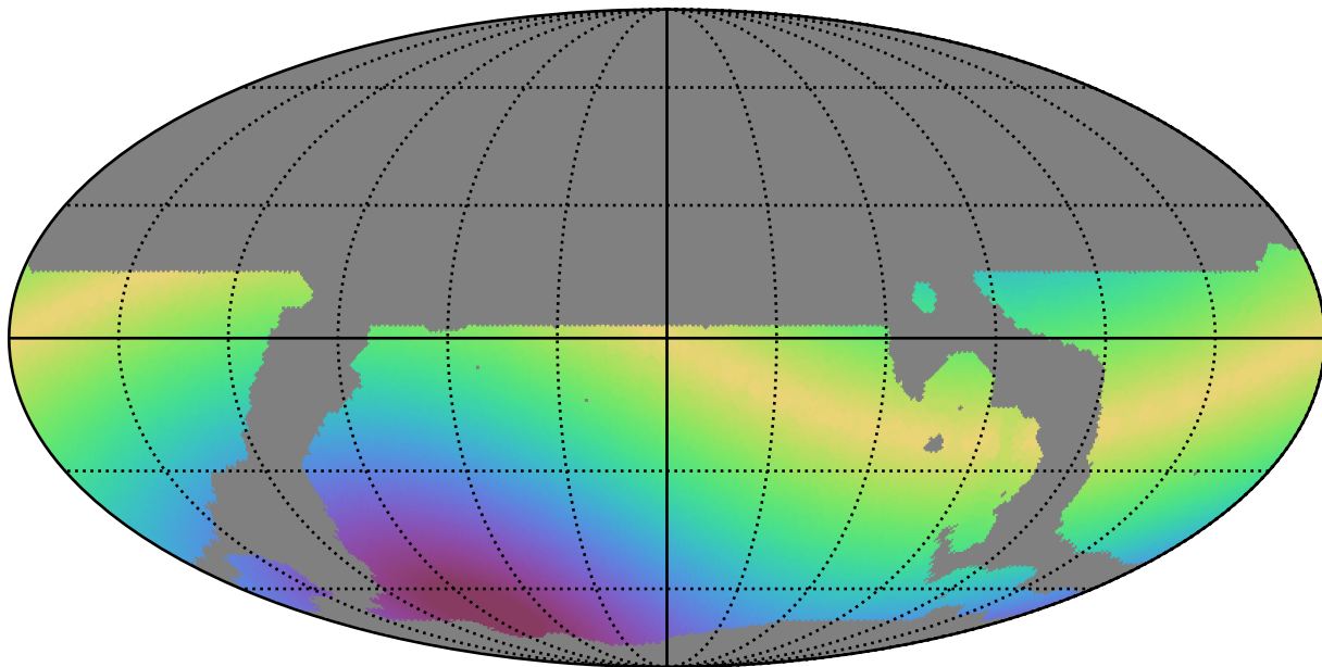
weather_cloudso4v3.4_10yrs WFD z band: Max solarElong
