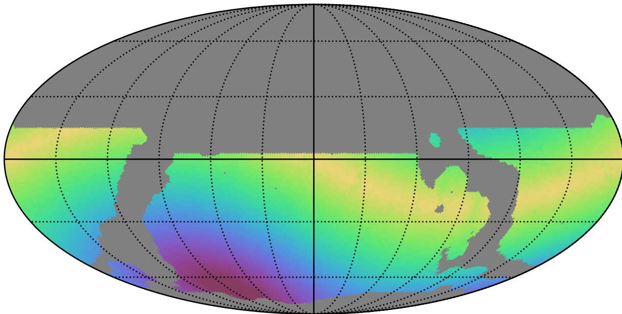
weather_cloudso4v3.4_10yrs WFD u band: Max solarElong
