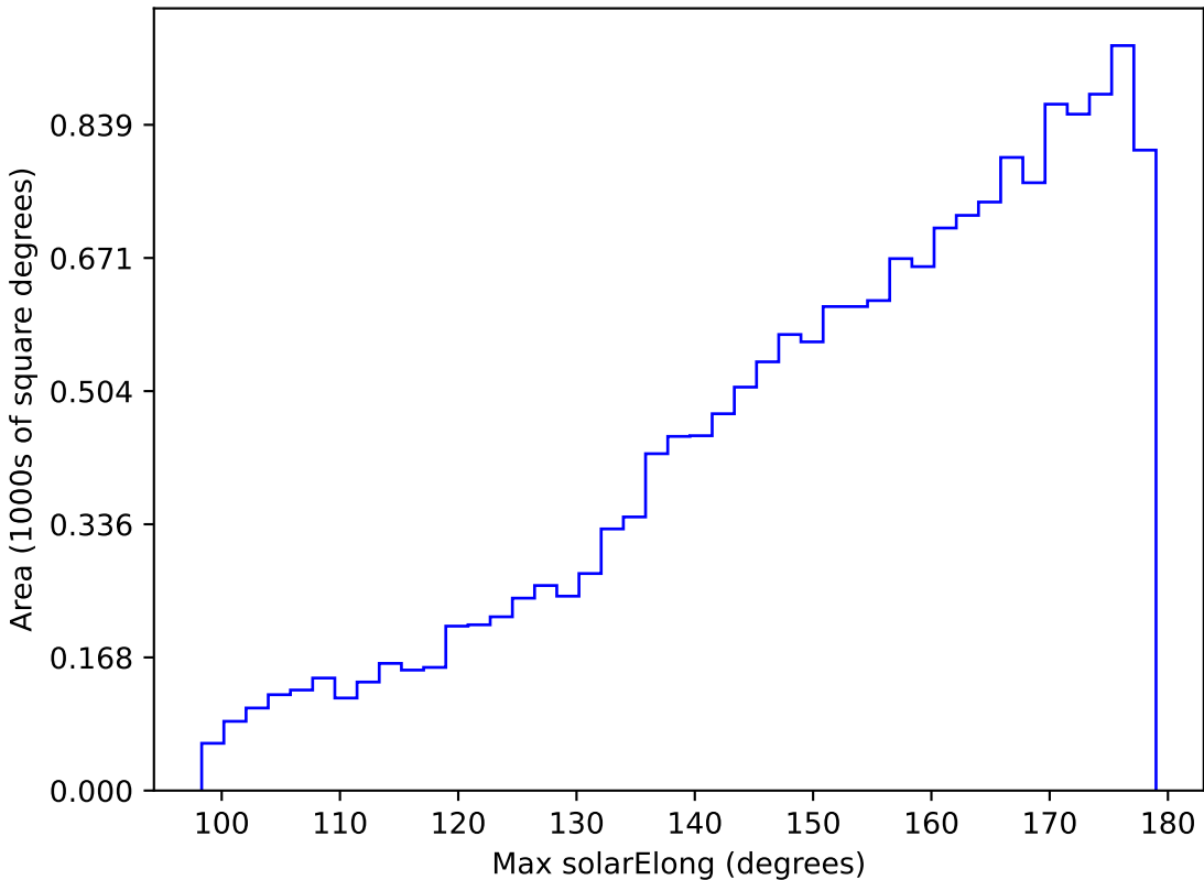
weather_cloudso4v3.4_10yrs WFD u band: Max solarElong
