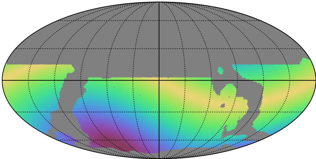
weather_cloudso4v3.4_10yrs WFD r band: Max solarElong
