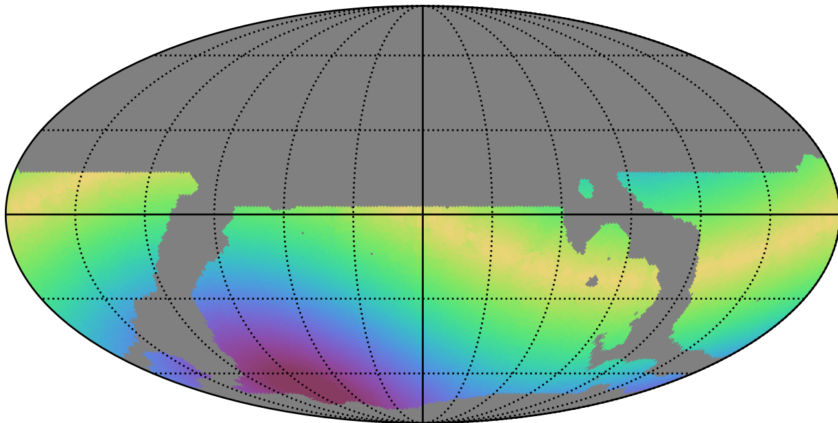
weather_cloudso4v3.4_10yrs WFD g band: Max solarElong
