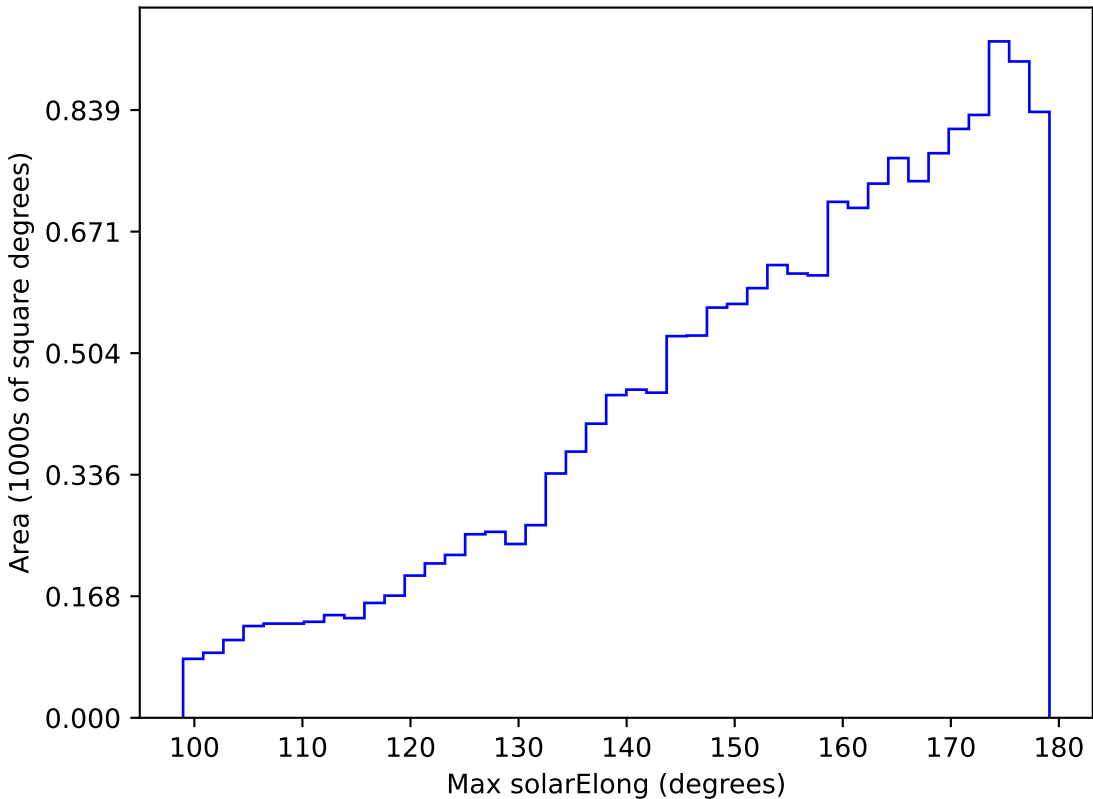
weather_cloudso4v3.4_10yrs WFD g band: Max solarElong
