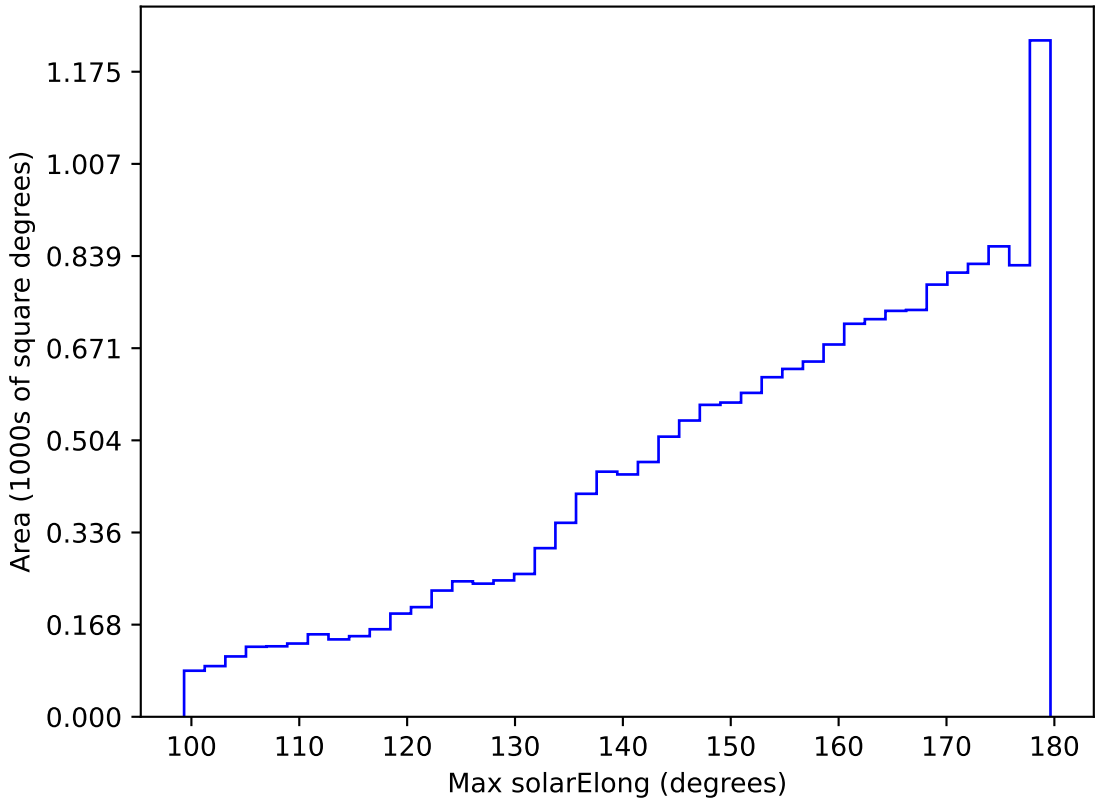
weather_cloudso4v3.4_10yrs WFD all bands: Max solarElong
