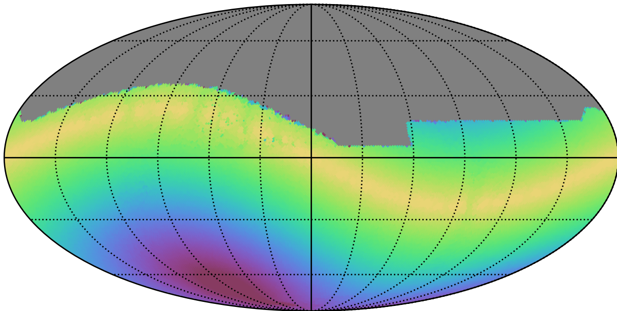
weather_cloudso4v3.4_10yrs All sky z band: Max solarElong
