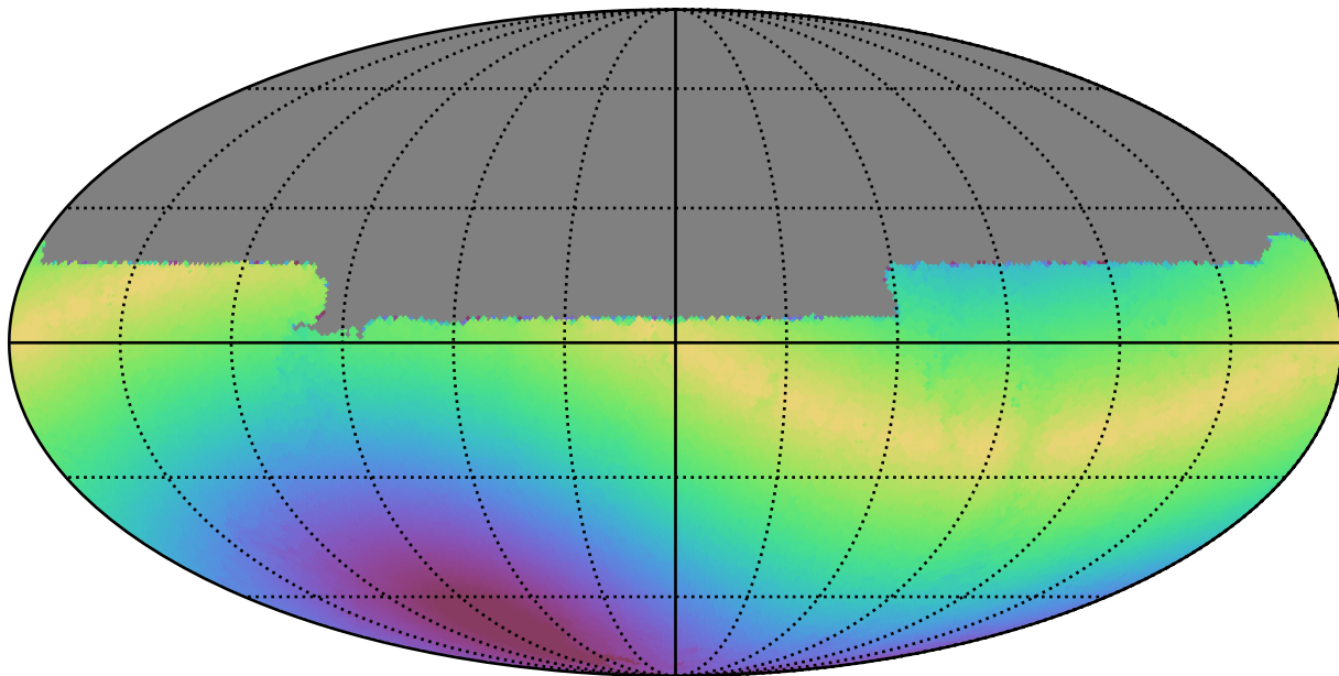
weather_cloudso4v3.4_10yrs All sky u band: Max solarElong
