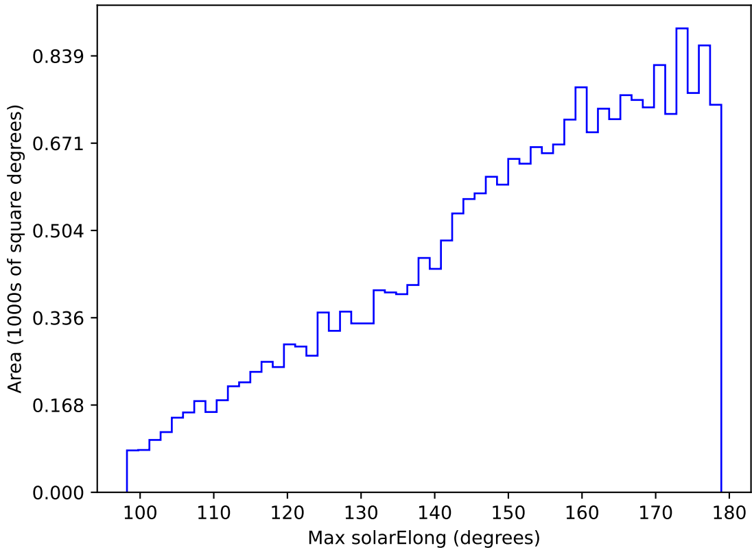
weather_cloudso4v3.4_10yrs All sky u band: Max solarElong
