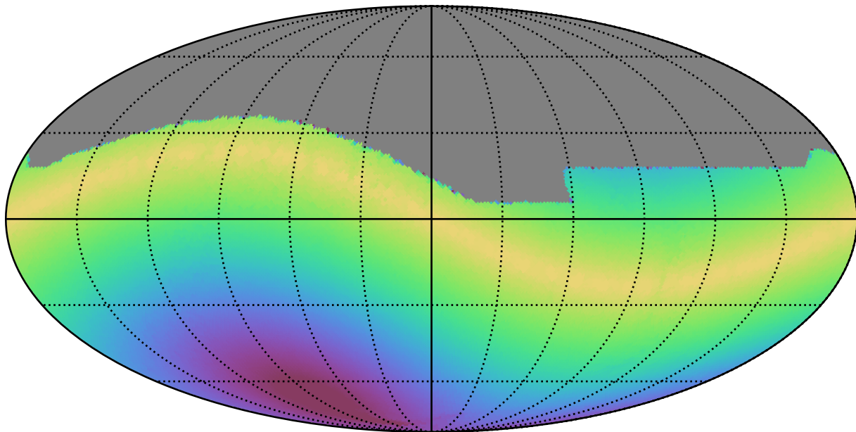
weather_cloudso4v3.4_10yrs All sky r band: Max solarElong
