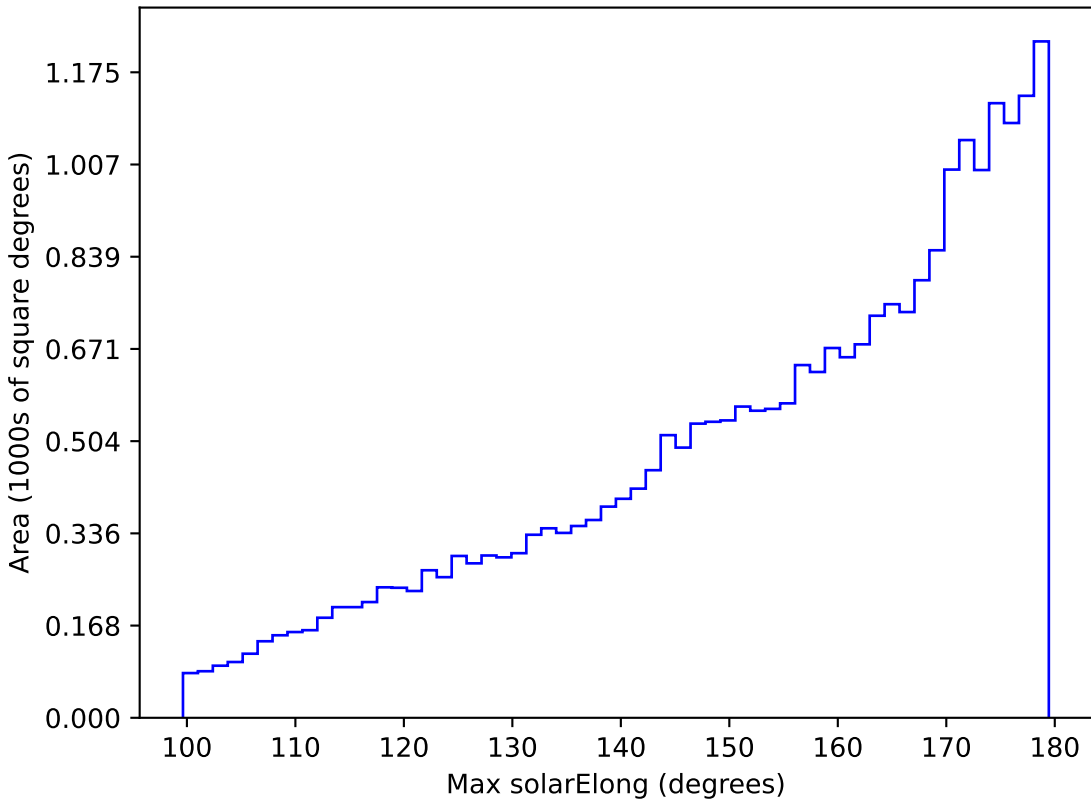
weather_cloudso4v3.4_10yrs All sky r band: Max solarElong
