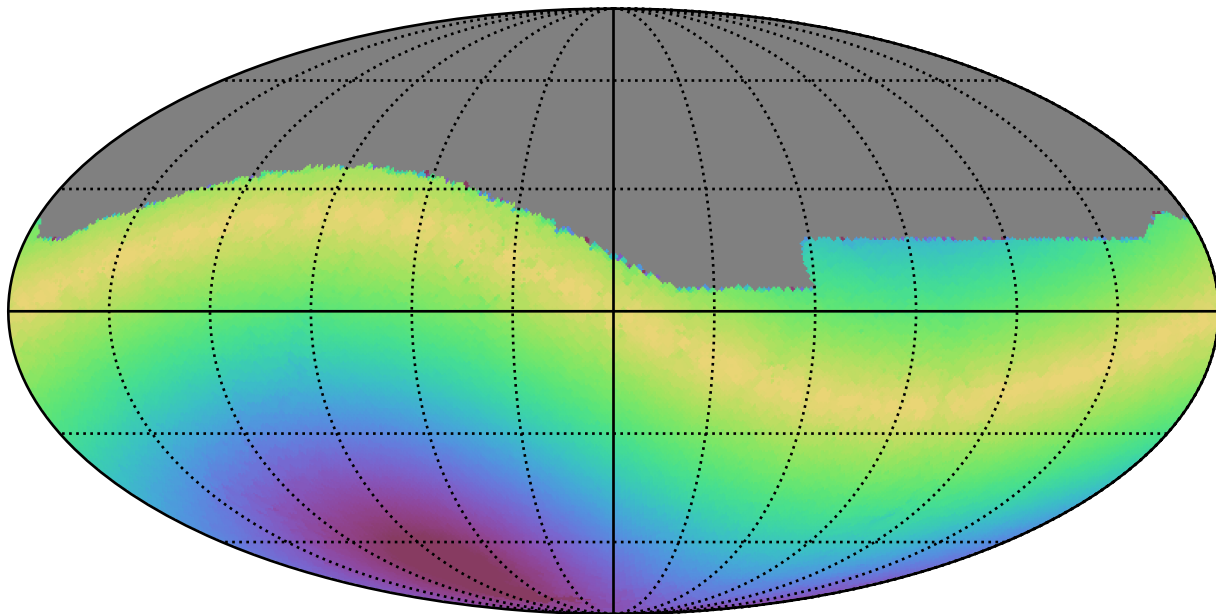
weather_cloudso4v3.4_10yrs All sky g band: Max solarElong
