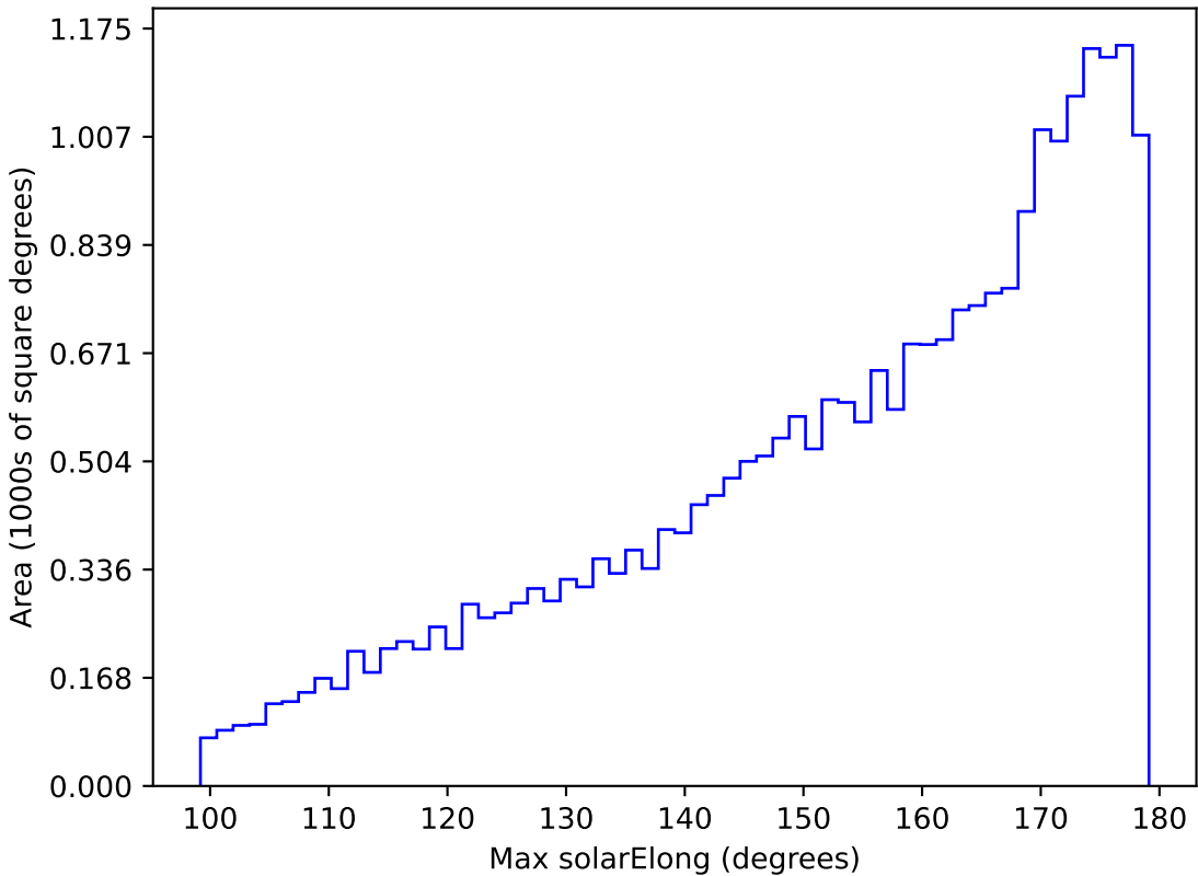
weather_cloudso4v3.4_10yrs All sky g band: Max solarElong
