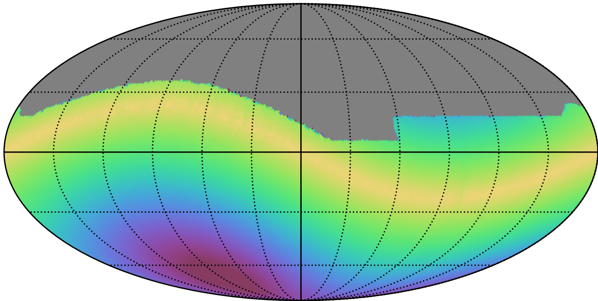
weather_cloudso4v3.4_10yrs All sky all bands: Max solarElong
