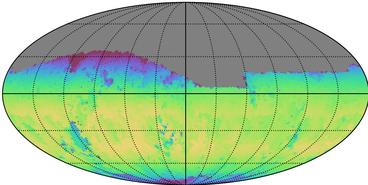
weather_cloudso4v3.4_10yrs Yr 1 z band: Max skyBrightness
