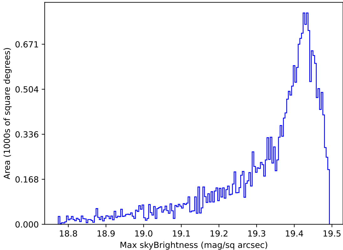
weather_cloudso4v3.4_10yrs Yr 1 z band: Max skyBrightness
