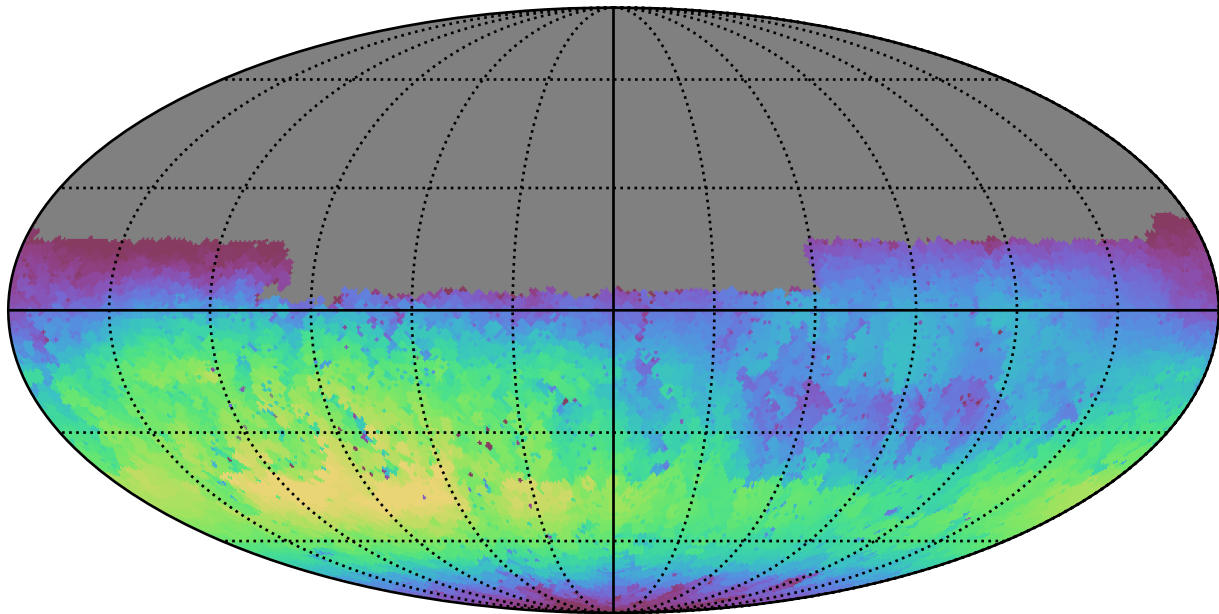
weather_cloudso4v3.4_10yrs Yr 1 u band: Max skyBrightness
