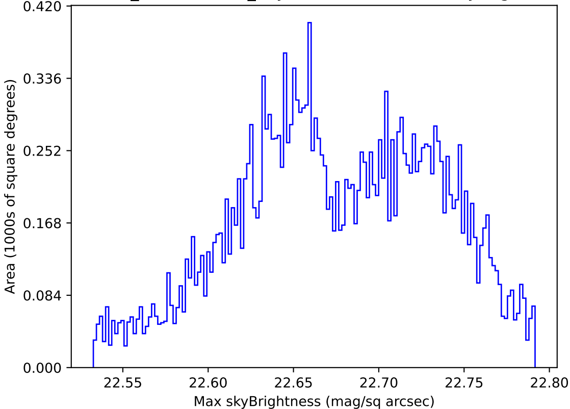
weather_cloudso4v3.4_10yrs Yr 1 u band: Max skyBrightness
