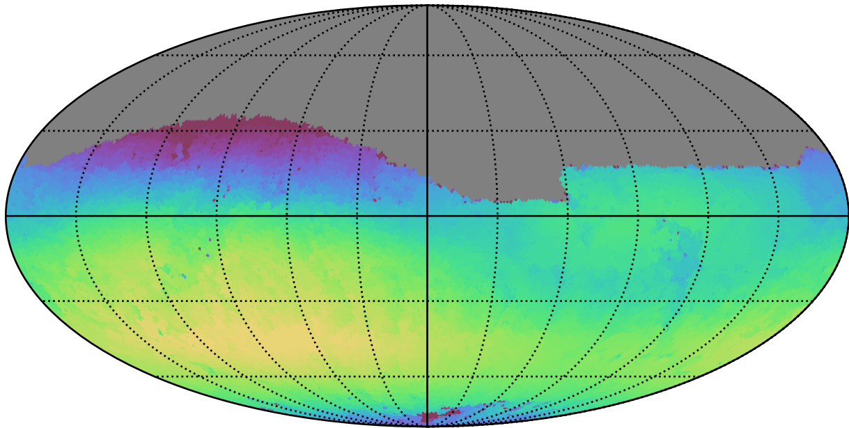
weather_cloudso4v3.4_10yrs Yr 1 r band: Max skyBrightness
