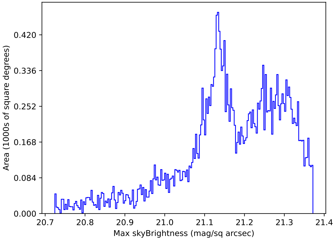
weather_cloudso4v3.4_10yrs Yr 1 r band: Max skyBrightness
