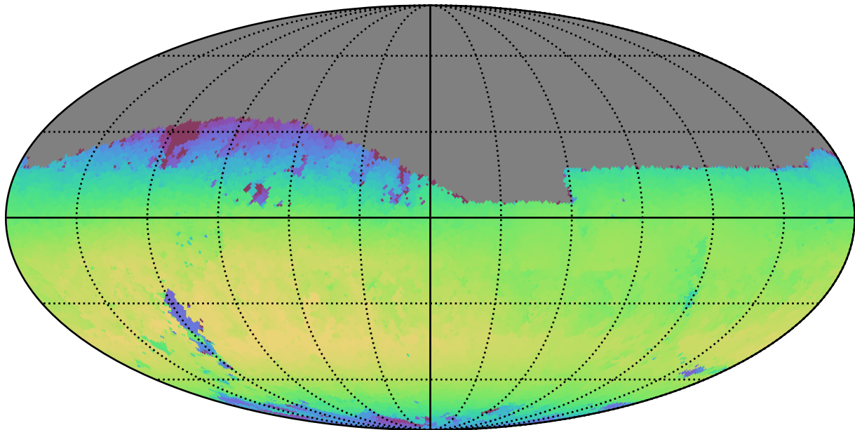
weather_cloudso4v3.4_10yrs Yr 1 i band: Max skyBrightness
