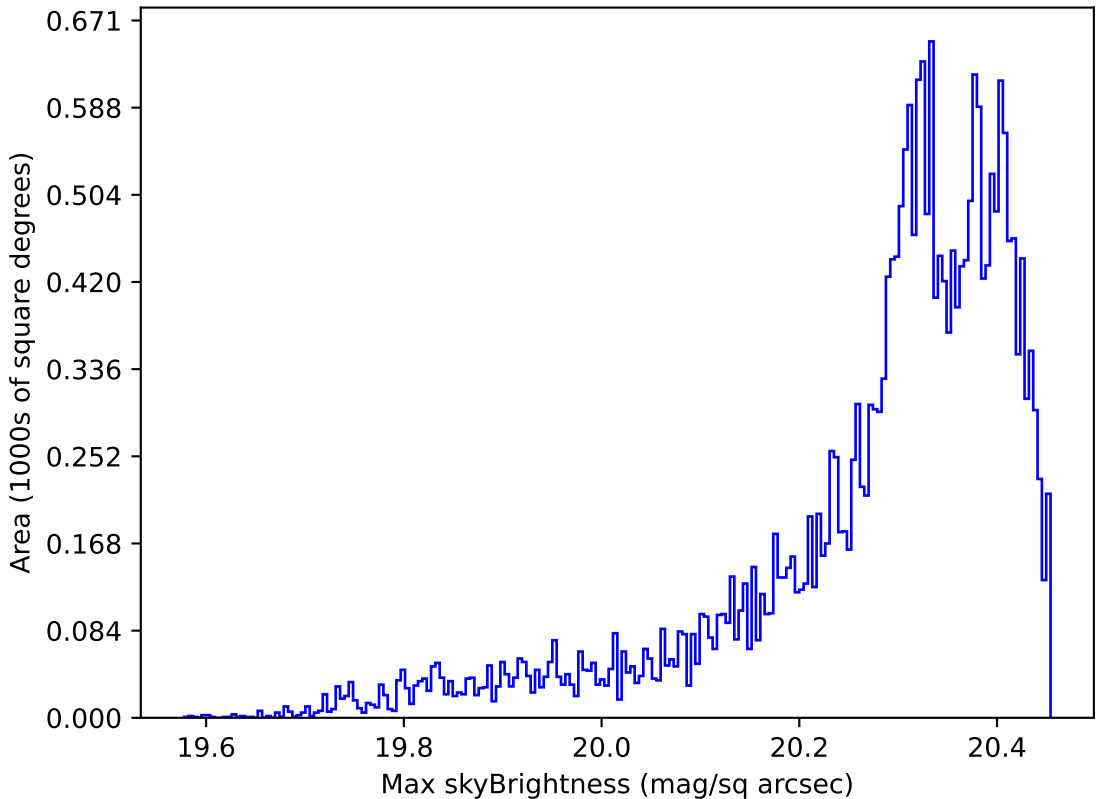
weather_cloudso4v3.4_10yrs Yr 1 i band: Max skyBrightness
