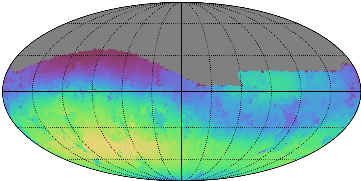
weather_cloudso4v3.4_10yrs Yr 1 g band: Max skyBrightness
